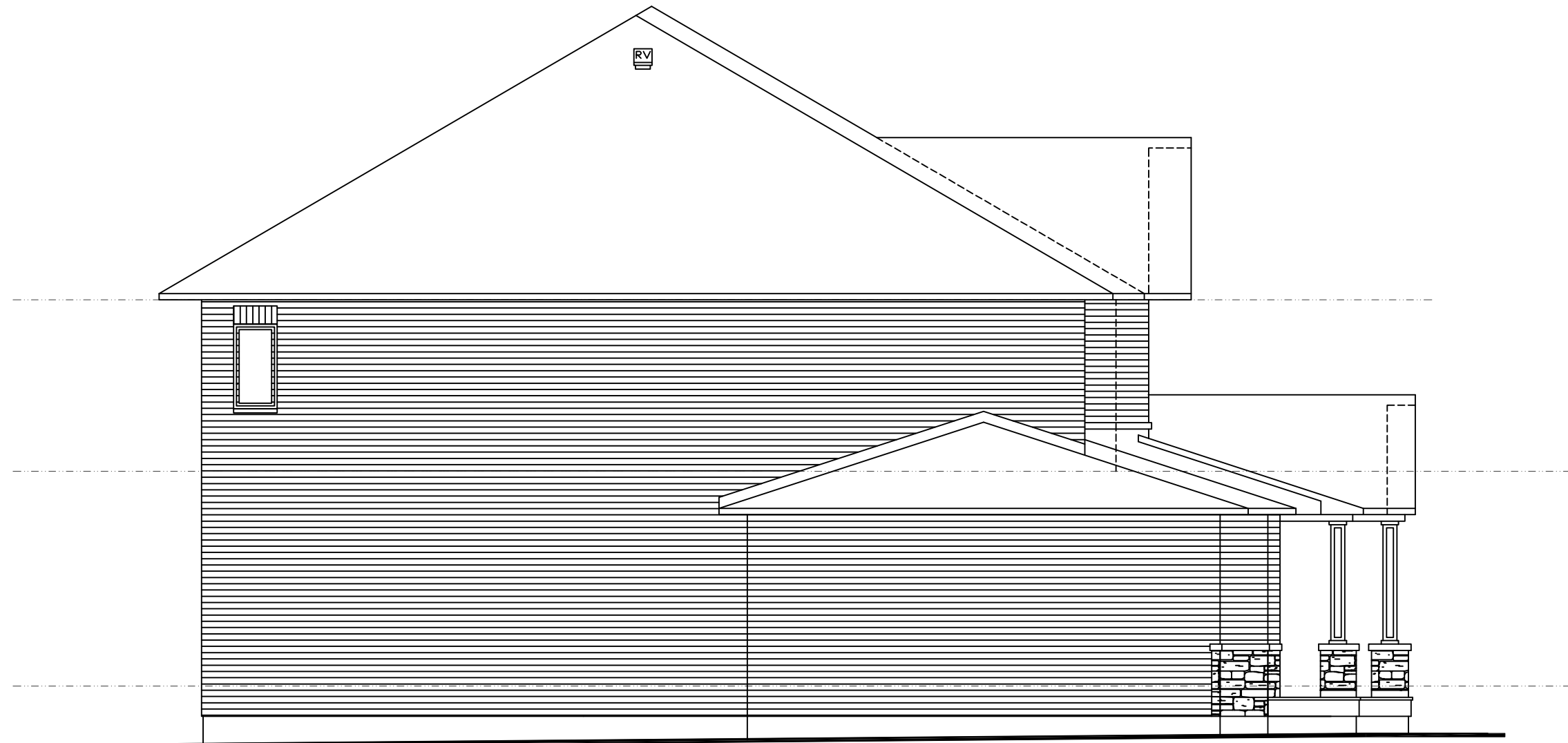
LEFT ELEVATION VERSAILLES 3 CAR BUTTERNUT CREEK LOT 4
